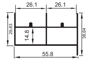
7005 H 0.740 kg/m Alt ve Yan Ray
